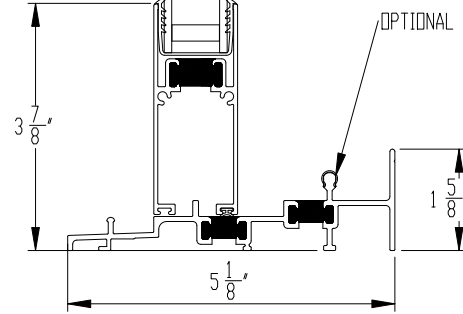
4 FIXED SILL
