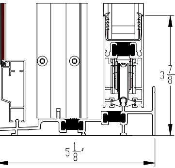
5 MOVING PANEL SILL
