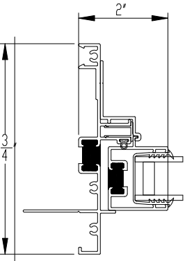
1 FIXED PANEL JAMB
