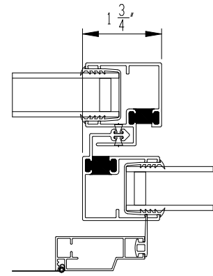
3 MEETING RAILS
