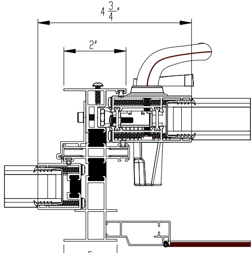
2 MOVING & FIXED PANEL JAMB
