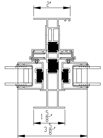
3 FIXED & FIXED PANEL JAMB
