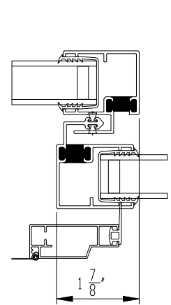
2 MOVING & FIXED PANEL JAMB
