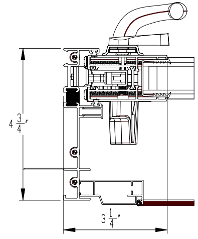
1 MOVING PANEL JAMB
