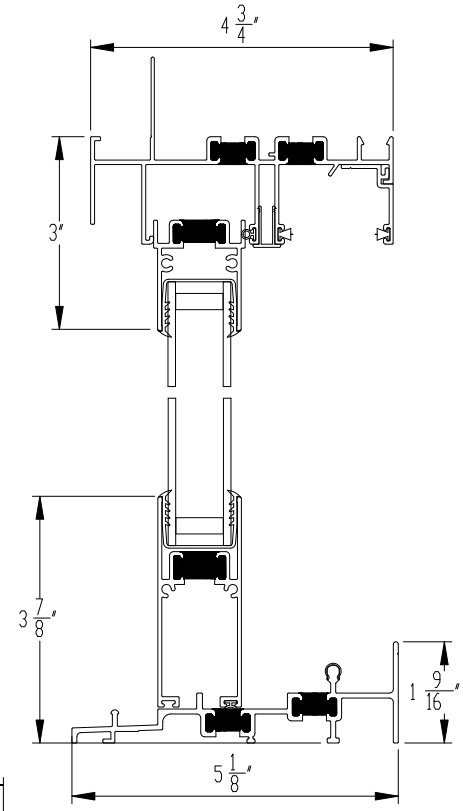
4 FIXED SILL
