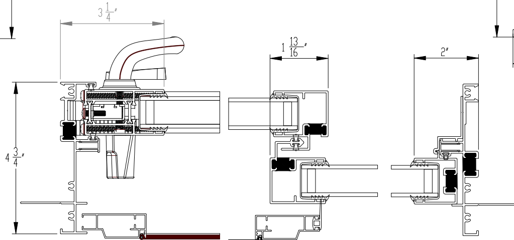
1 MOVING PANEL JAMB
