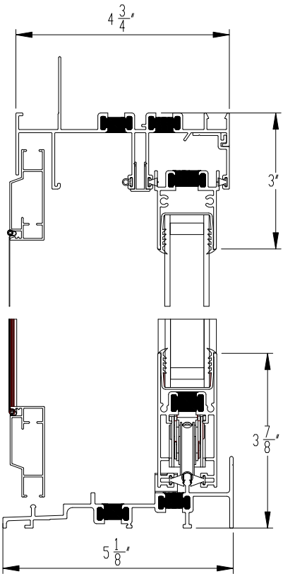
6 MOVING PANEL HEAD
