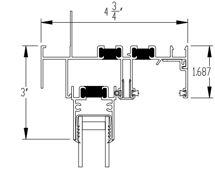
7 FIXED HEAD
