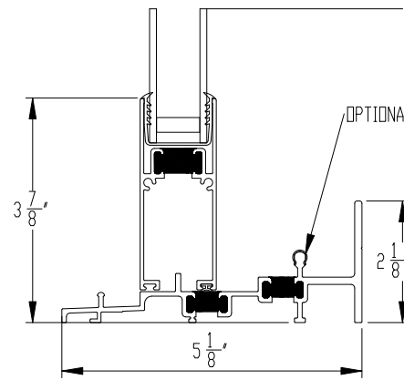
4 FIXED SILL
