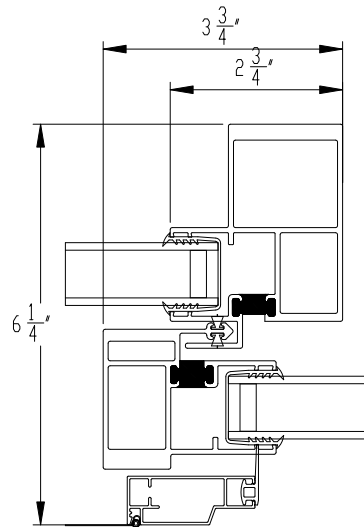
3 MEETING RAILS
