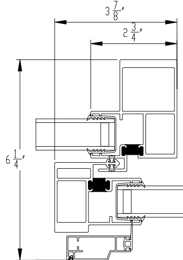
2 MEETING RAILS
